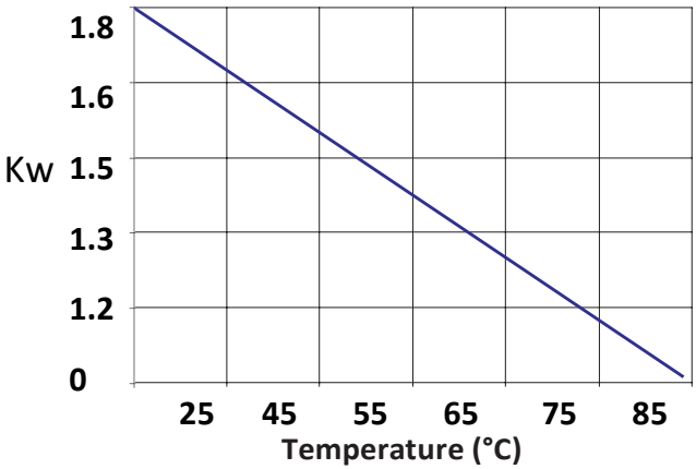
Load Power Derating vs. Ambient Temperature
