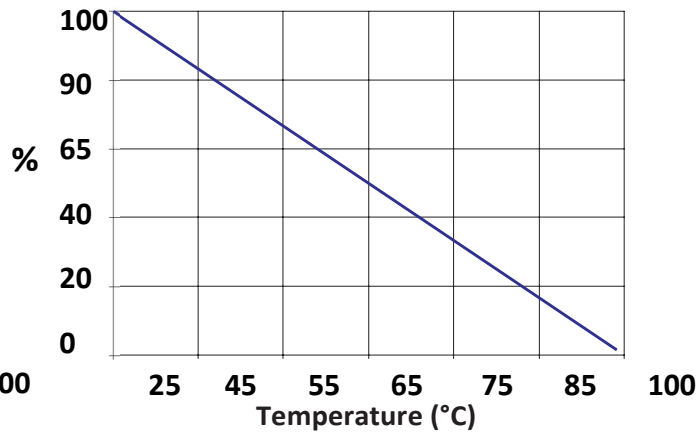
Load Power Derating vs. Ambient Temperature
